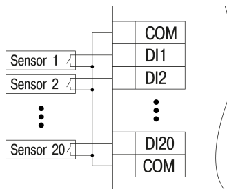
Fig. 5 Contact sensor wiring (MV210-204)
