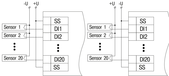
Fig. 3 Contact sensor wiring (MV210-202) – option 1
