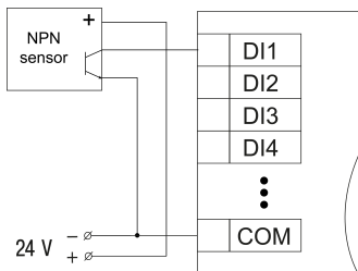
Fig. 8 NPN sensor wiring (MV210-204)
