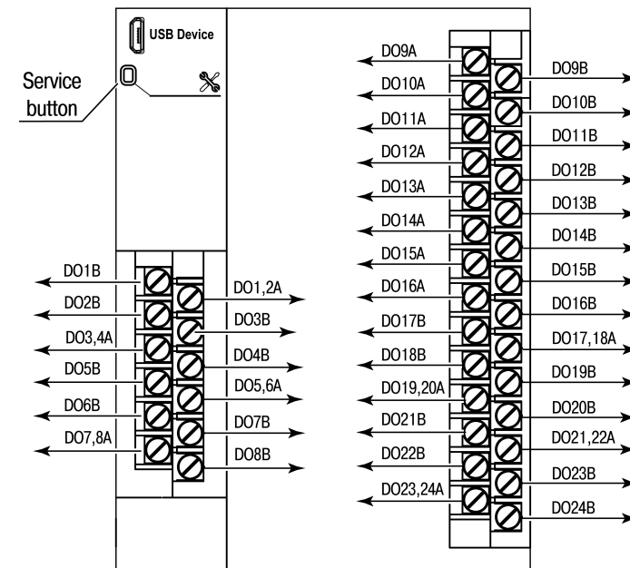
Fig. 2 Terminal block layout
