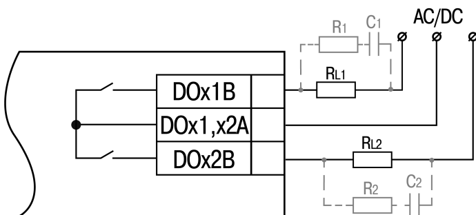
Fig. 4 Relay wiring (common contact)
